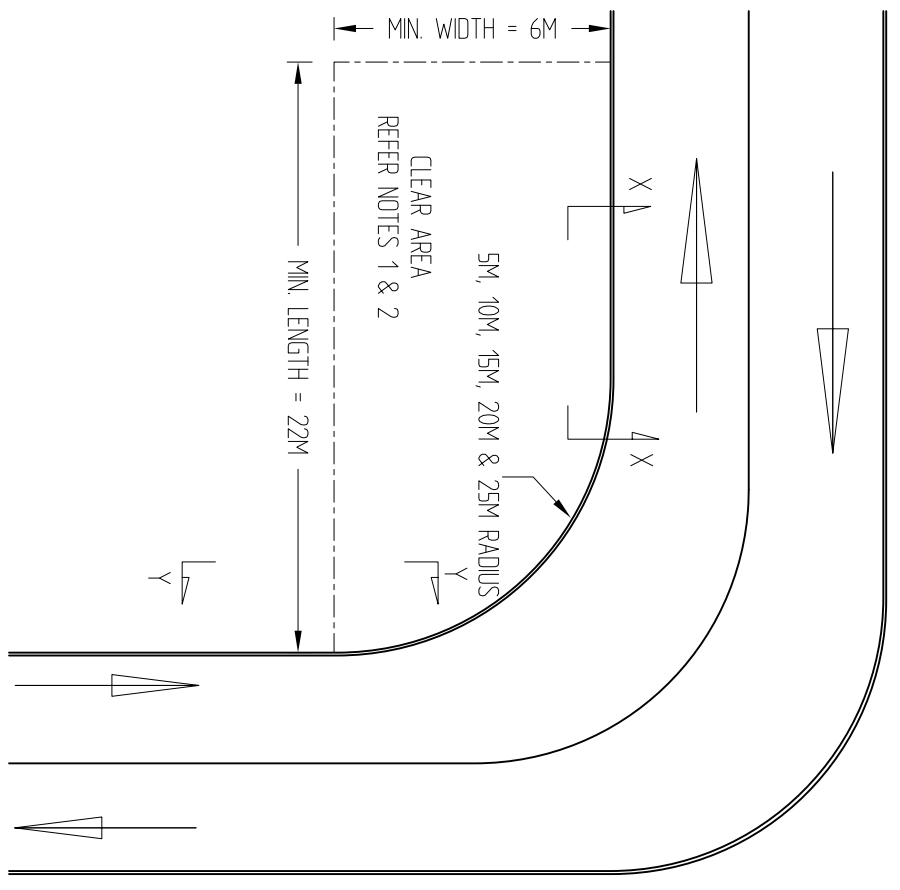
TYPICAL CURVED RAIL LAYOUT
