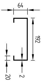
TYPICAL HANDRAIL CROSS SECTION SCALE 1:10
