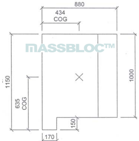
Standard Unit (Section B-B)
