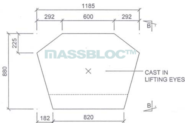
Standard Plan View
