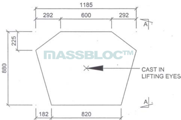
Base Plan View
