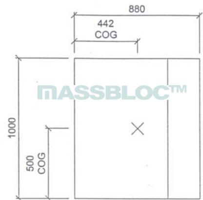
Base Unit (Section A-A)
